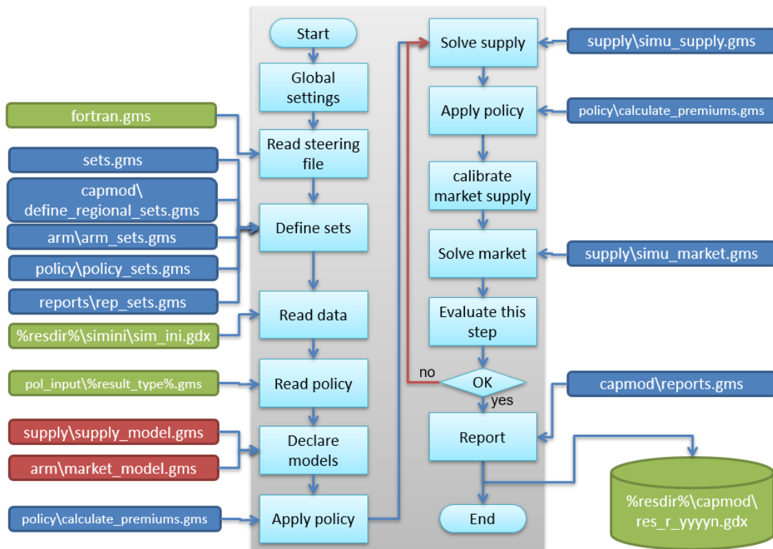
Figure 10: Program flow of capmod.gms
