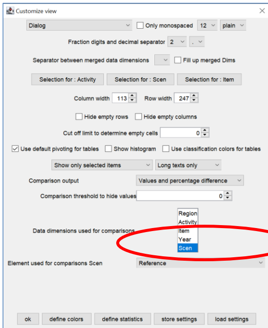
Figure 38: View comparisons of scenarios
