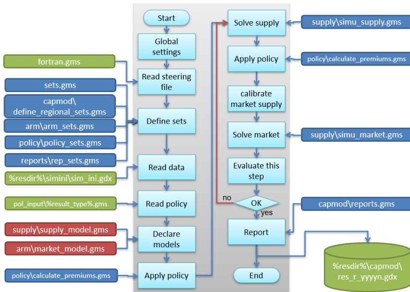
Figure 10: Program flow of capmod.gms
