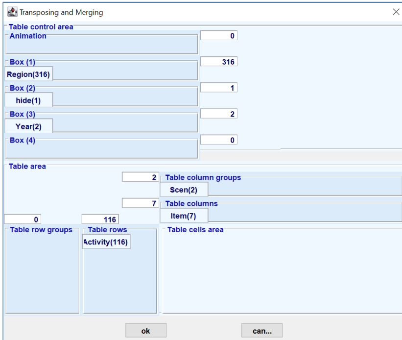
Figure 37: Changing dimensions of a table
