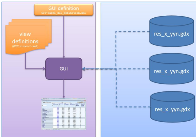
Figure 9: Viewing results from GAMS in the GUI
