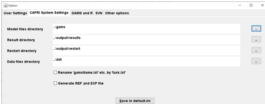
Figure 15: CAPRI System Settings
