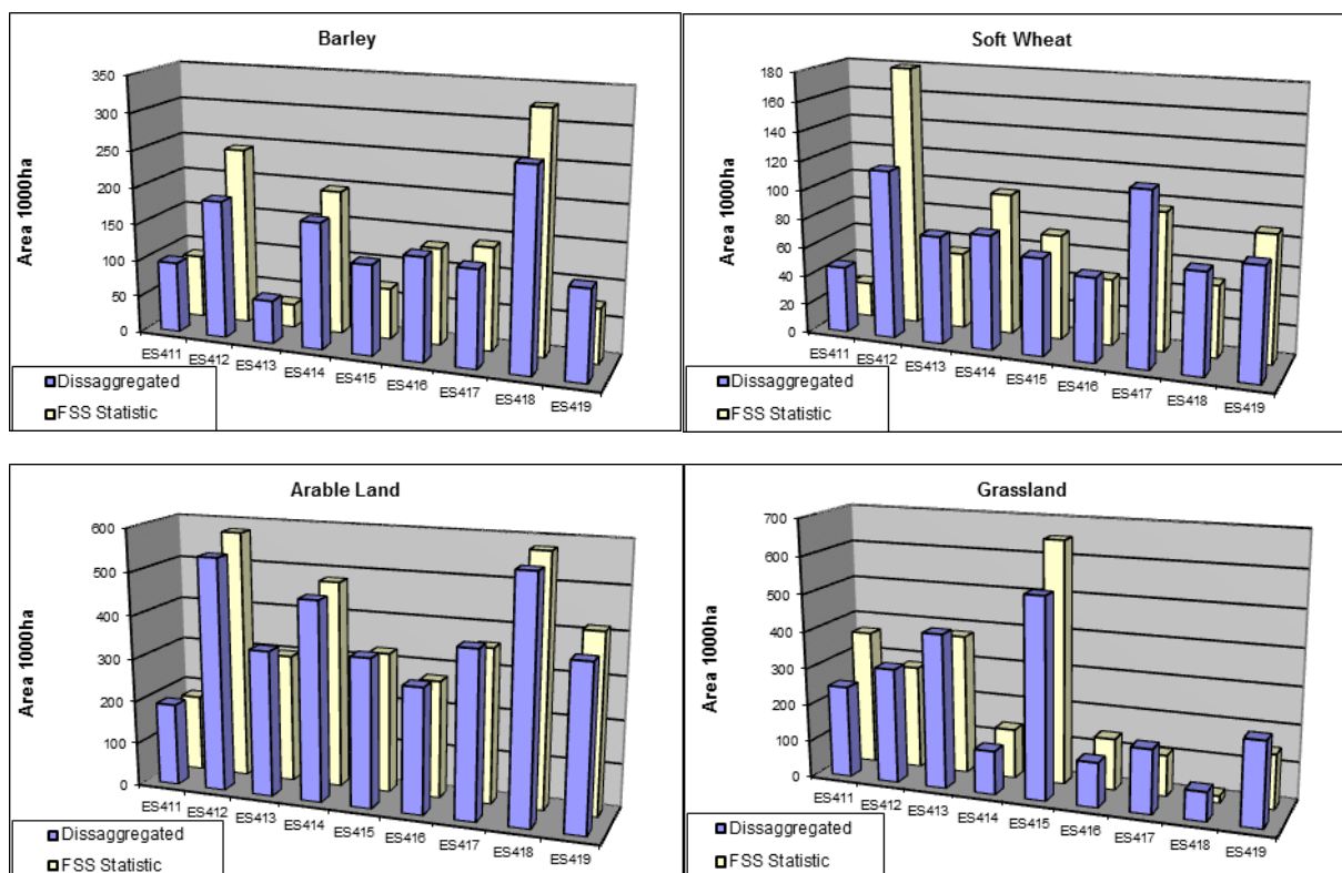
Figure 25. Comparison of estimated and observed shares in NUTS III region for different crops (Castilla Leon ES410)
