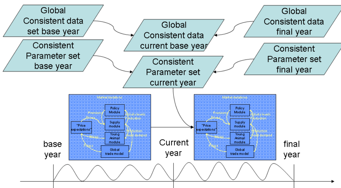
Figure 20. Calibration process of the recursive-dynamic version
