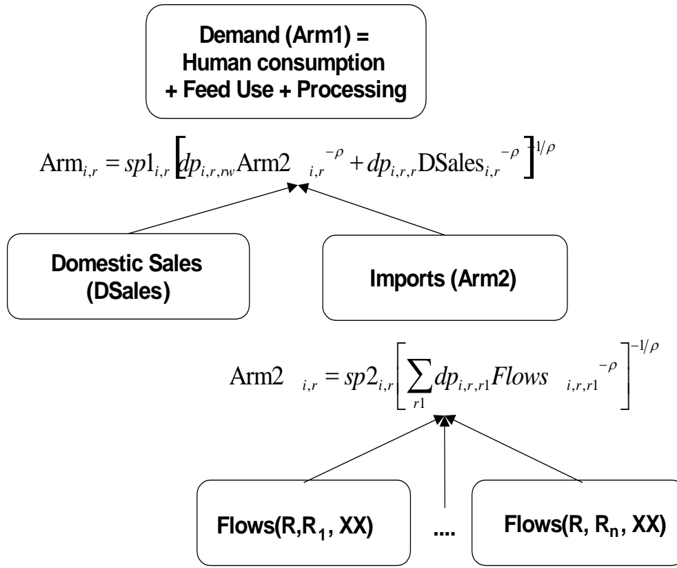
Figure 8. Two-stage Armington System
