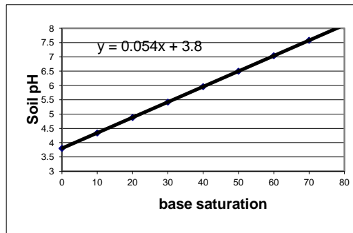
Figure 33. Linear relationship between soil pH and base saturation
