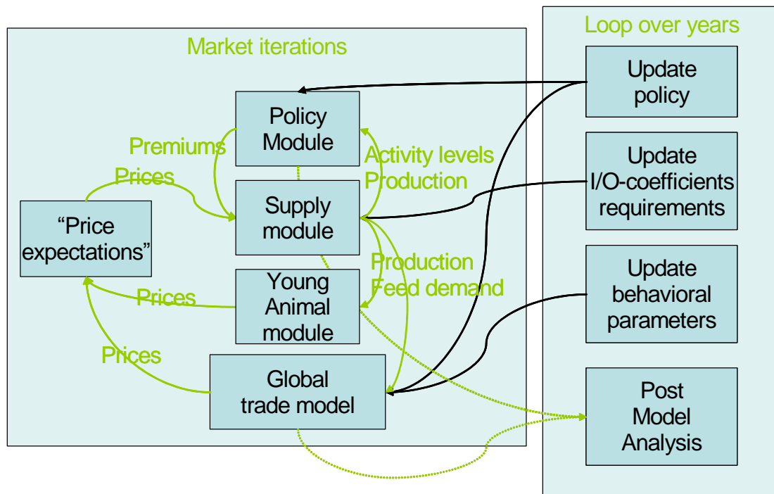
Figure 19. General layout of the recursive dynamic version
