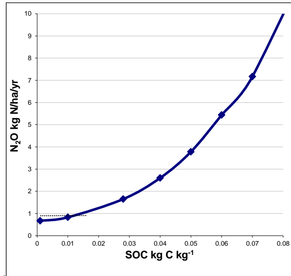
Figure 32. DNDC model sensitivity to SOC
